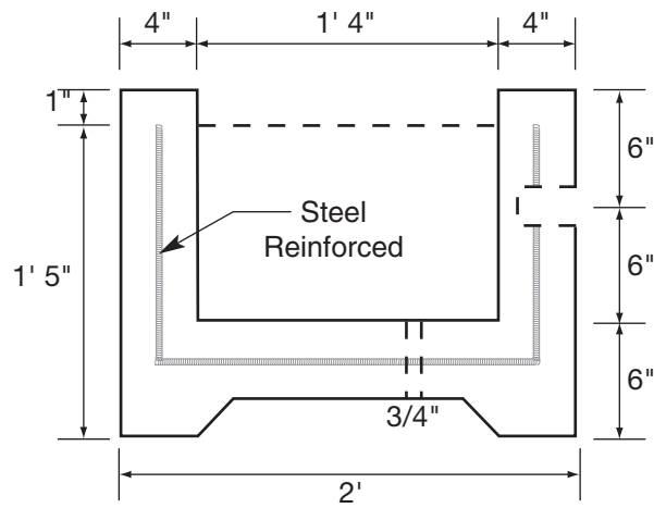
SECTION VIEW
